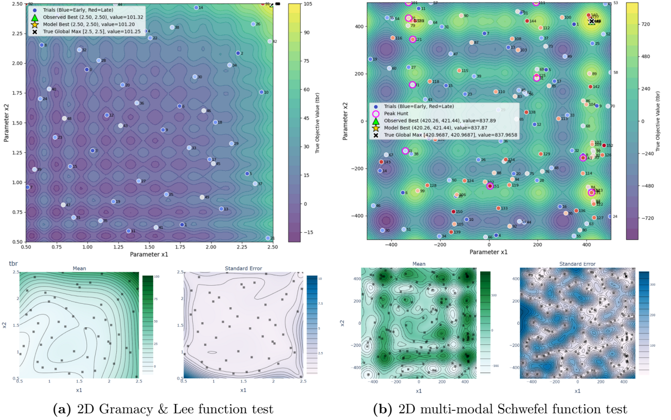
Figure 3: Benchmarking of the ML optimisation algorithm across challenging mathematical landscapes. (a) 2D Gramacy & Lee function test. (b) 2D multi-modal Schwefel function test. Pink markers annotate where a secondary “peak hunt” is triggered. Both used N = 150 trials (including N_{sobol} = 50 ), with UCB \beta = 1,000,000 , \epsilon = 0.75 , and n_{hunt} = 10 .
