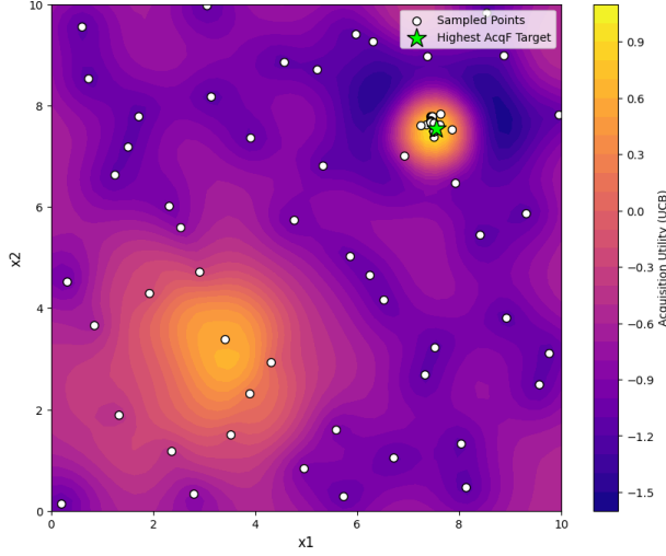
(a) Explorative tuning ( \beta = 1,000,000 )
