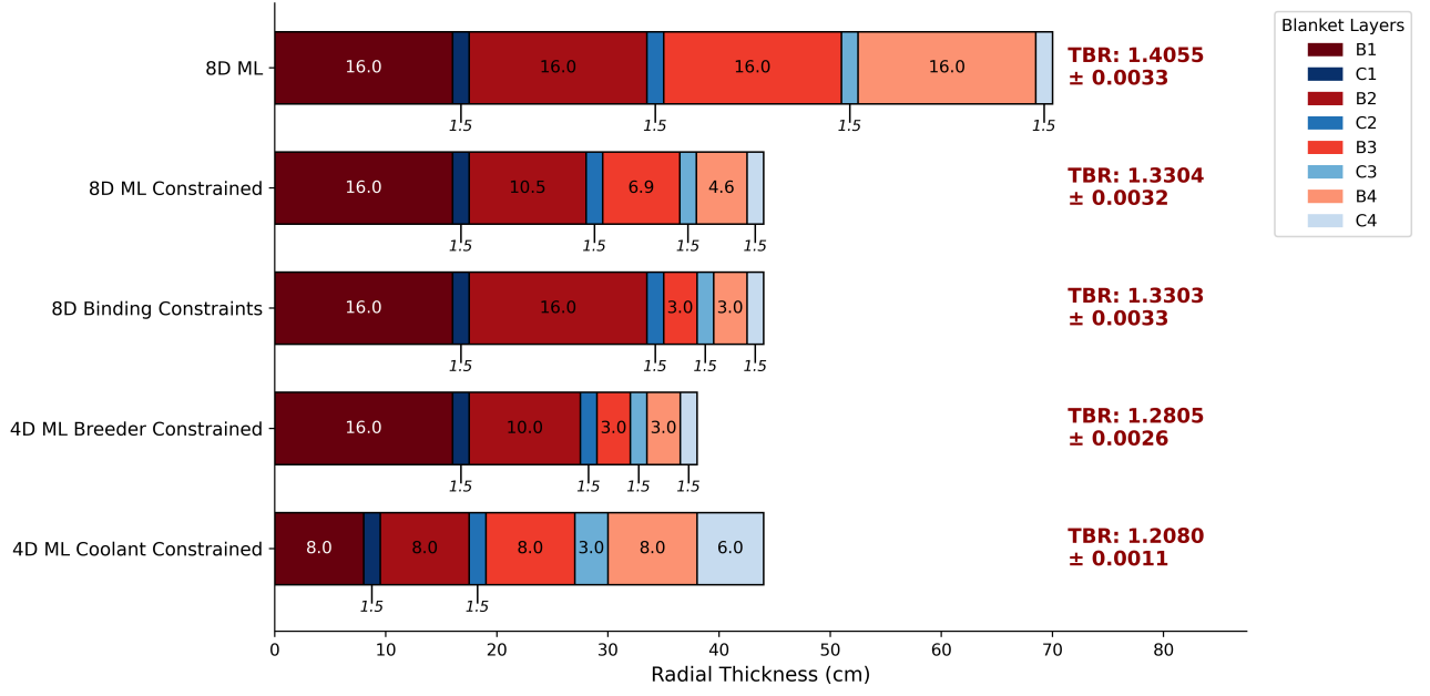
Figure 10: Radial thickness profiles and resulting global TBR for the ML optimised TBR-thickness studies detailed in Section 4.3.3. Associated TBR values are annotated alongside their standard statistical uncertainty. N = 100 was used for all except for unconstrained 8D N = 150 , where these include N_{sobol} = 50 . Hyper-parameters \epsilon = 0.5 and \beta = 1,000,000 were tuned for these studies.
