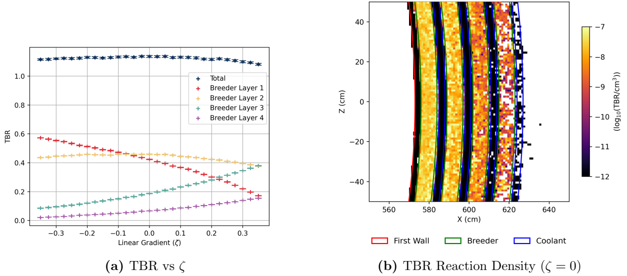
Figure 5: (a) Global and layer-specific TBR performance against \zeta , paired with a heatmap of breeding reactions (b).
