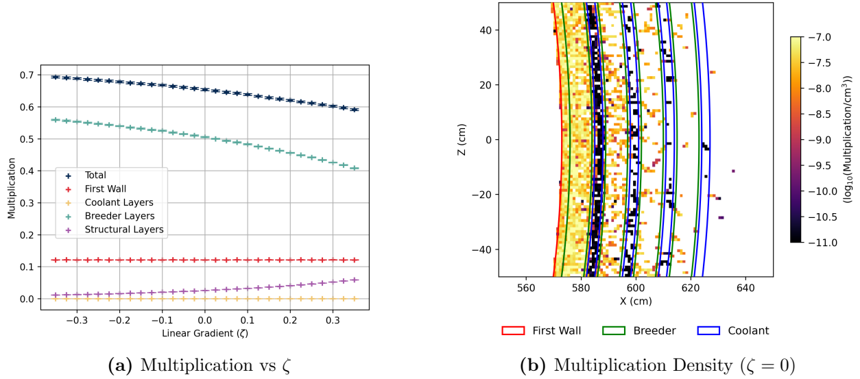
Figure 7: (a) Total neutron multiplication rate per source neutron split between reactor component, alongside the spatial concentration in the plasma-facing layers (b).
