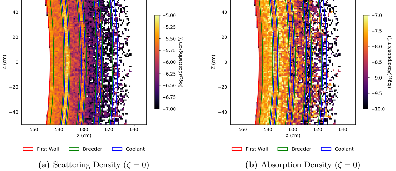
Figure 8: Heat maps of scattering (a) and total absorption interactions (b) in the reactor wall. Absorption tally records all absorptions, including breeding, spallation and parasitic reactions.
