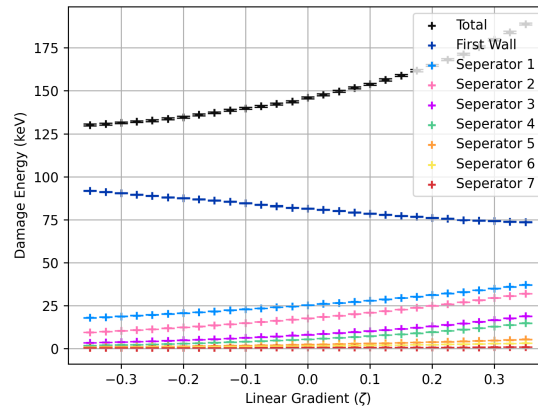
Figure C3: Total damage energy deposited into the plasma-facing first wall and internal structural separators across the geometric gradient.
