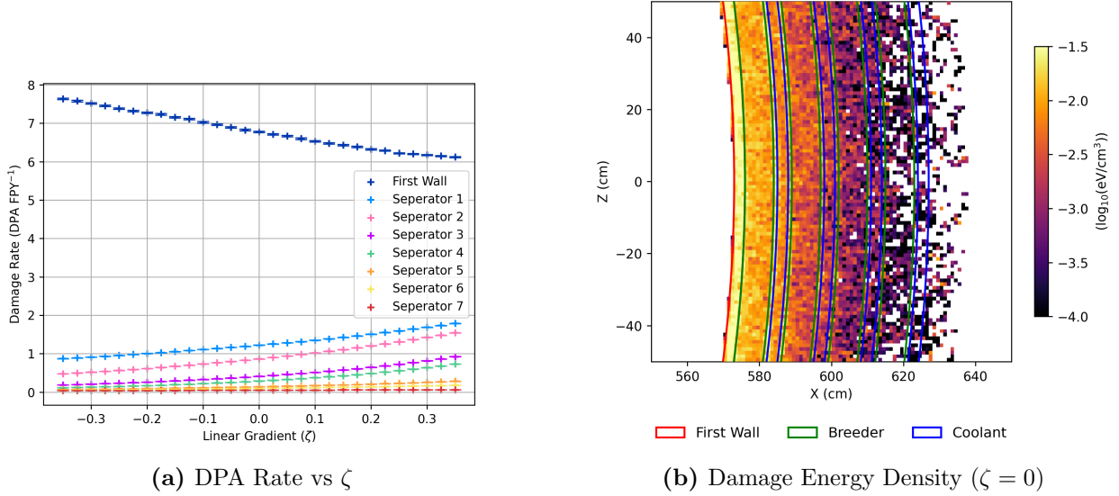
Figure 9: Radiation damage metrics across the linear gradient alongside the spatial profile of damage energy deposition.
